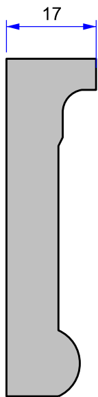
Profile
